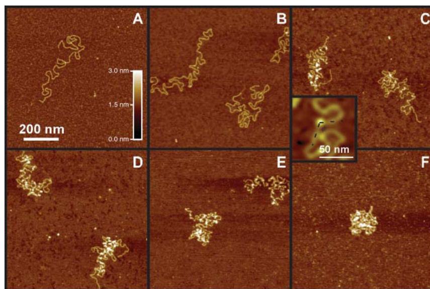
FIGURE 1 AFM images of linearized pBR322 DNA molecules after exposure to increasing concentrations of Abf2p (ratio of Abf2p/bp in parentheses). (A) No Abf2p; (B) 1.5 \mu\text{g/mL} (1:20); (C) 3.5 \mu\text{g/mL} (1:8); (D) 7 \mu\text{g/mL} (1:4); (E) 15 \mu\text{g/mL} (1:2); and (F) 25 \mu\text{g/mL} (1:1). ( Inset ) Closeup image of a bend in the DNA backbone induced by the bound protein ( bright dot ).
