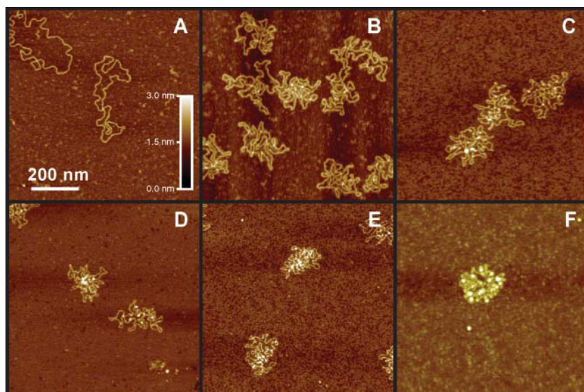
FIGURE 2 AFM images of relaxed circular pBR322 DNA molecules after exposure to increasing concentrations of Abf2p (ratio of Abf2p/bp in parentheses). (A) No Abf2p; (B) 1.5 \mu\text{g/mL} (1:20); (C) 3.5 \mu\text{g/mL} (1:8); (D) 7 \mu\text{g/mL} (1:4); (E) 15 \mu\text{g/mL} (1:2); and (F) 25 \mu\text{g/mL} (1:1).
